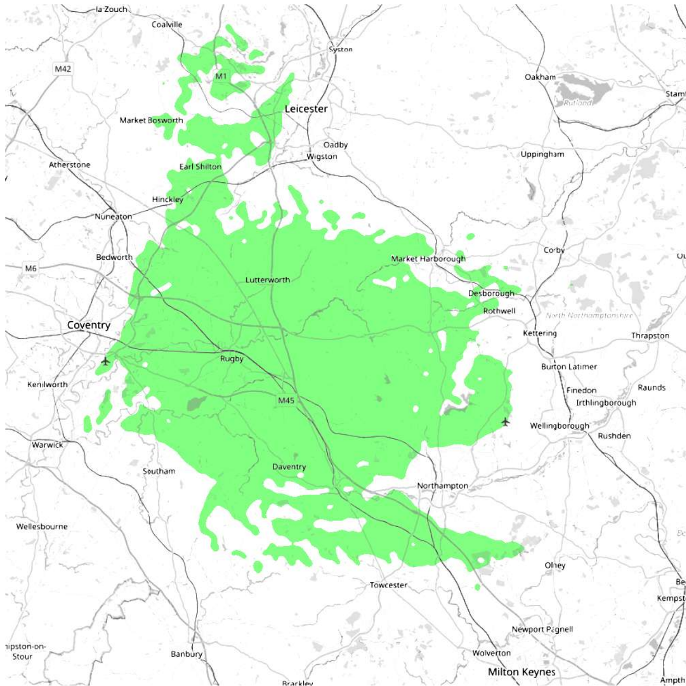
Rugby+Daventry SSDAB Coverage map – calibrated using drive test data
